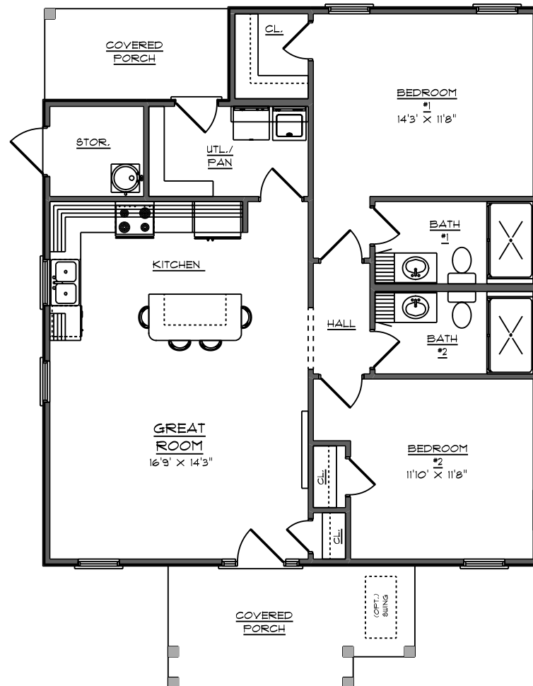
FLOOR PLAN
